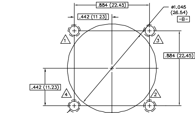
4-HOLE MOUNTING PATTERN
