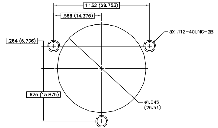
3-HOLE MOUNTING PATTERN
