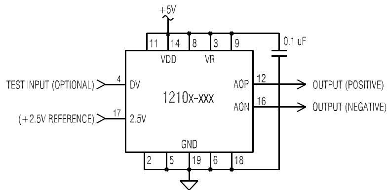
RECOMMENDED CONNECTIONS
