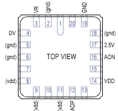
PINOUT (LCC & JLC PACKAGES)
